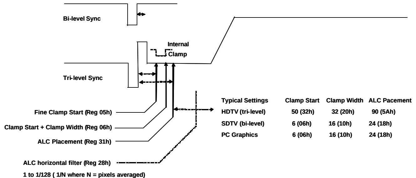
Figure 15. Clamp Placement
